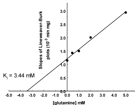
Figure 2. Secondary plot of Lineweaver–Burk slopes for the determination of the apparent K_i of glutamine inhibition of the colorimetric enzymatic reaction of L- \gamma -glutamyl- p -nitroanilide. See Experimental for details.
