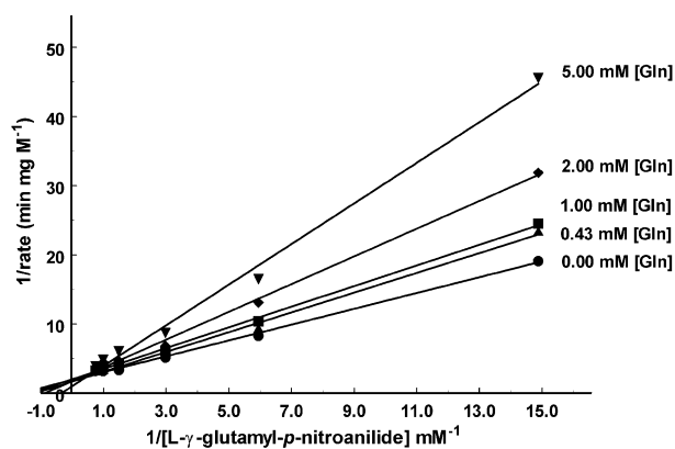
Figure 1. Lineweaver–Burk plots for the apparent inhibition of the colorimetric enzymatic reaction of L- \gamma -glutamyl- p -nitroanilide by glutamine. See Experimental for details.
